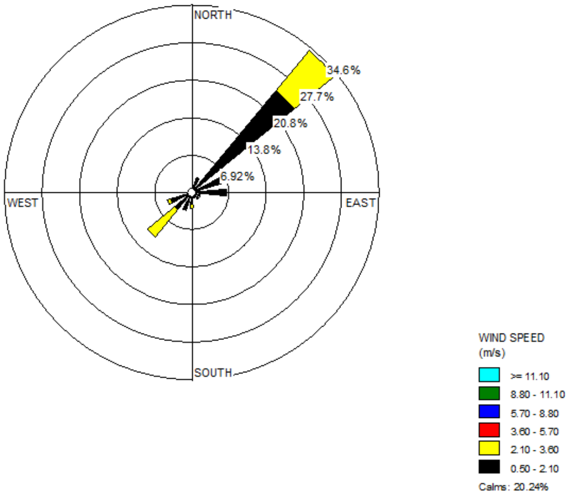
Figure 2-A – Wind Rose From 1838 Monitor
